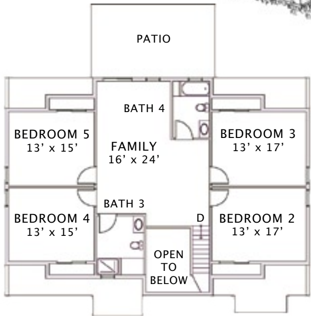
LOFT FLOOR
