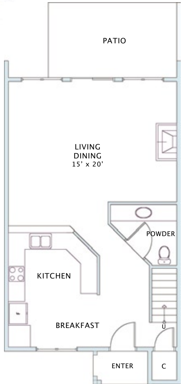
MAIN FLOOR
