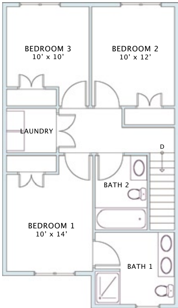
SECOND FLOOR
