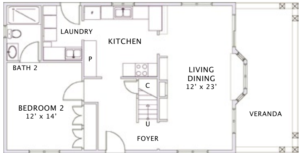
MAIN FLOOR
