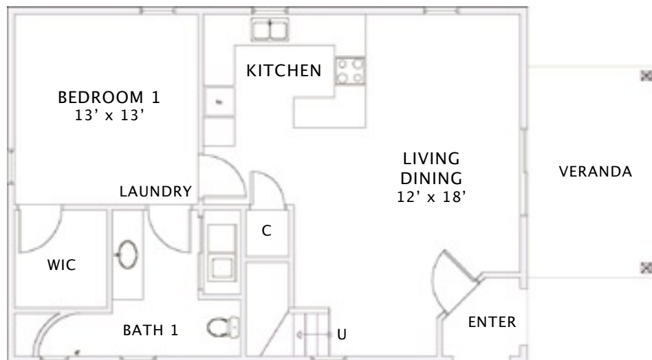
MAIN FLOOR
