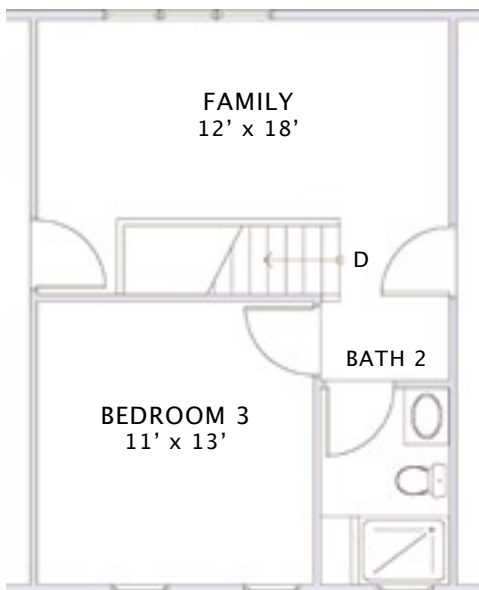
LOFT FLOOR
